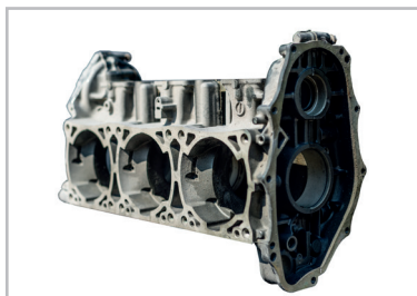
3-cylinder engine block
