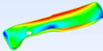
Analysis of the actual component by target/actual comparison of actual component to nominal component
